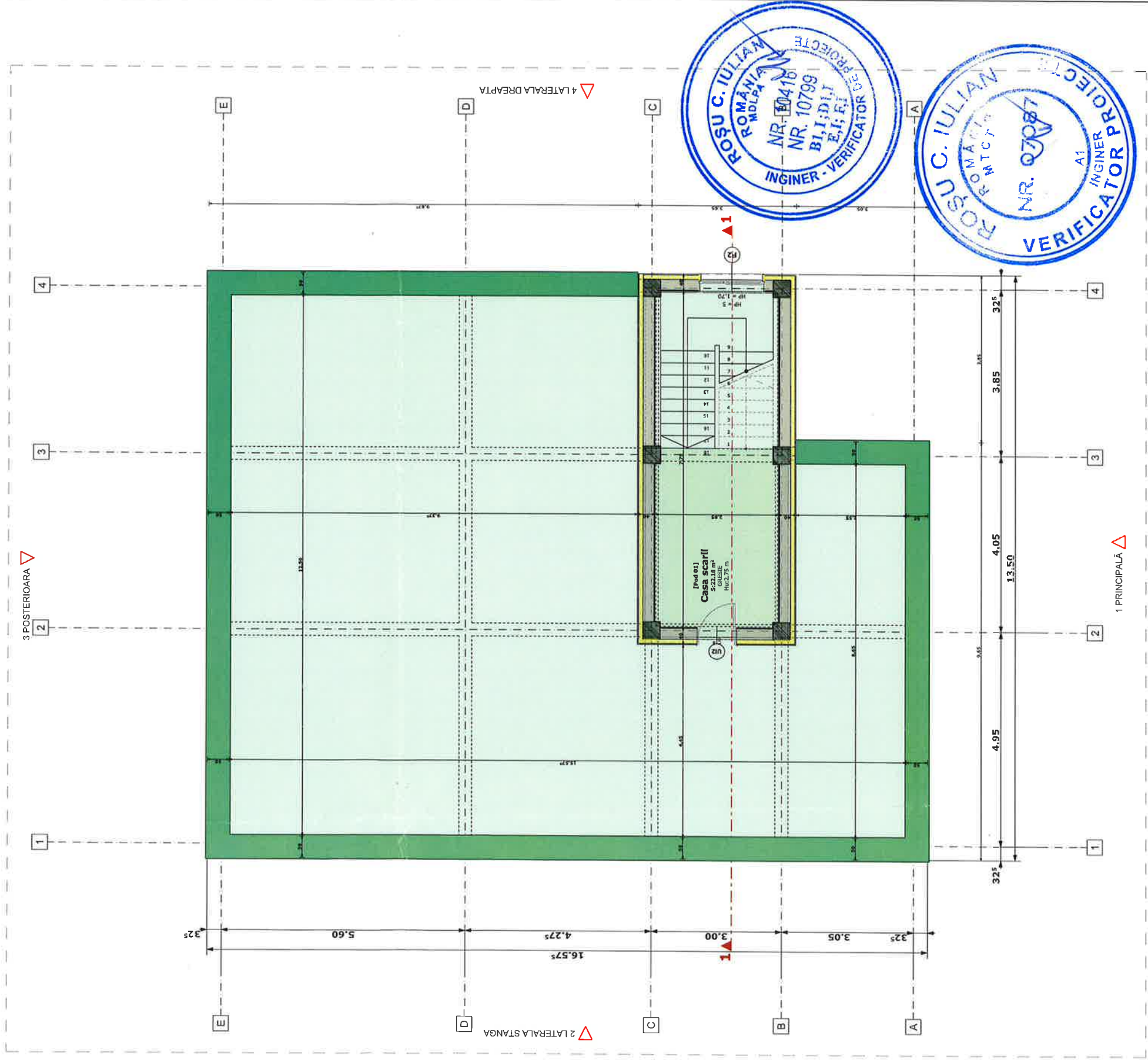
Plan terasa
